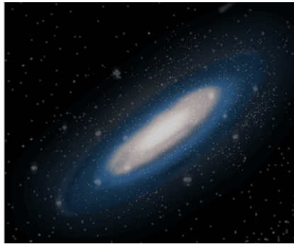
The Universe
