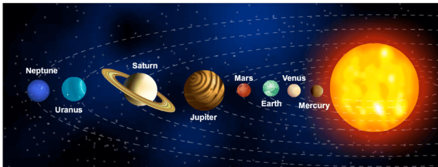
The Solar System
